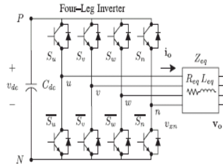
Fig. 3. Two-level four-leg PWM-VSI topology
