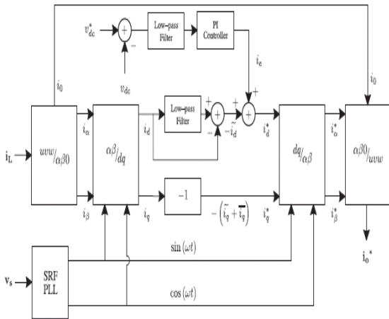
Fig. 5. dq -based current reference generator block diagram
