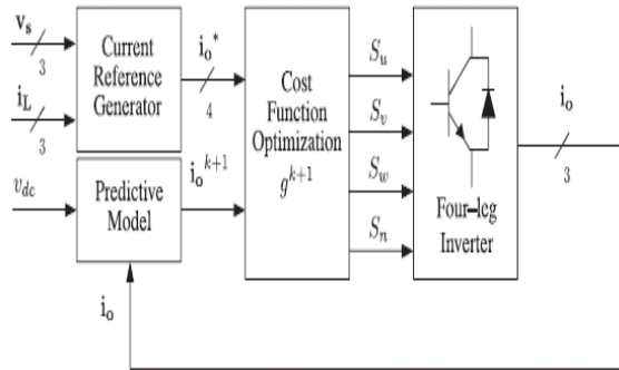
Fig. 4. Proposed predictive digital current control block diagram
