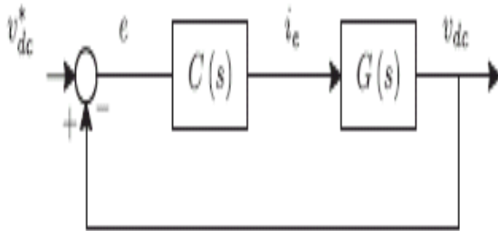
Fig. 7. DC-voltage control block diagram.
