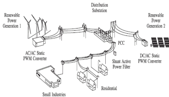
Fig. 1. Stand-alone hybrid power generation system with a shunt active power filter
