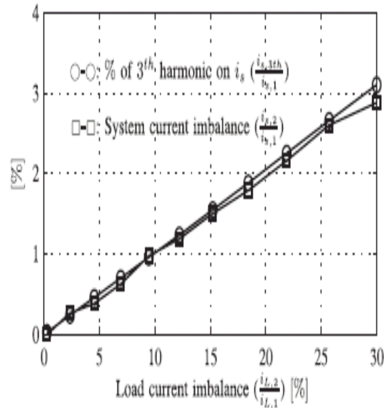
Fig. 6. Relationship between permissible unbalance load currents, the corresponding third-order harmonic content, and system current imbalance (with respect to positive sequence of the system current, i_s, 1 ).
