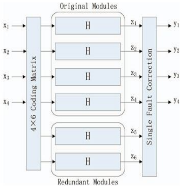
Fig. 2. Proposed coding scheme in general form
