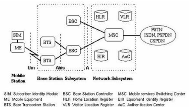
GSM architecture
