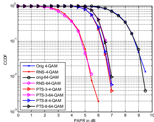
Figure1. PAPR reduction performance of the proposed scheme, PTS scheme and the conventional MIMO-OFDM
