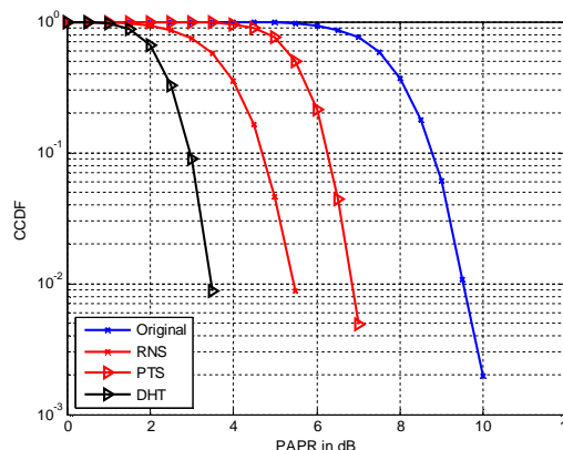
Figure2. PAPR reduction performance of extension scheme (DHT), RNS, PTS scheme of MIMO-OFDM.
