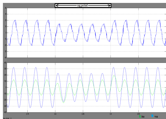
Fig. 4. Phase-a waveforms before, during, and after sag. (a) Load voltage. (b) Source voltage and source current (current is scaled up ten times for clear visibility).
