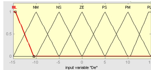
Fig 8. Membership function of voltage error
