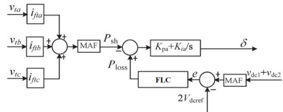
Fig. 2. Controller to calculate δ and P loss .
