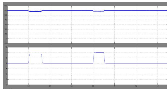
Fig.5. (a) Voltage across dc bus. (b) Load angle \delta .
