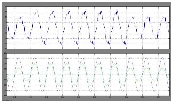
Fig. 3. Phase-a waveforms before, during, and after load change. (a) Load current. (b) Source voltage and source current (current is scaled up ten times for clear visibility).
