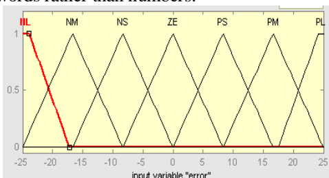
Fig 7. Membership function of voltage
