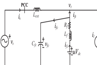
Fig.1. Single-phase equivalent circuit of DSTATCOM in a distribution network.
