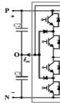
Fig. Basic npc circuit for single-phase
