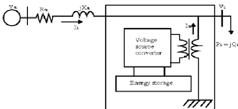
Fig . Basic DSTATCOM configurations
