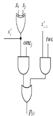
Fig. 3. Generation of the i-th bit p_{j,i} of the partial product PP_j for the conventional MB multiplier.
