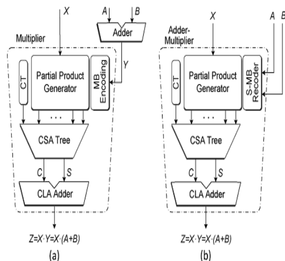
Fig. 1. AM operator based on the (a) conventional design and (b) fused design with direct recoding of the sum of A and B in its MB representation. The
