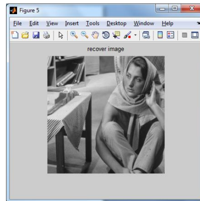
Figure 5: Input image
