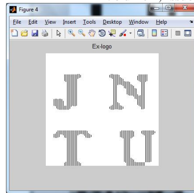
Figure 4: Ex-logo image
