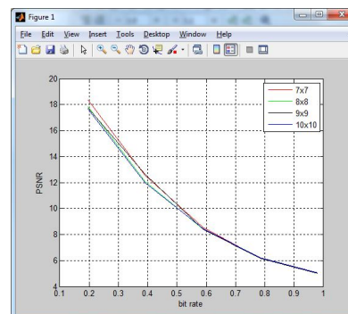
Figure 6: PSNR vs bit rate
