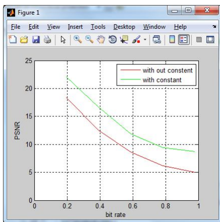
Figure 8: PSNR vs BER
