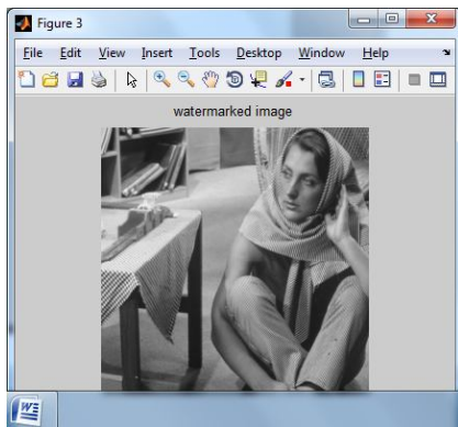
Figure 3: Watermarked image
