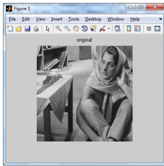
Figure 1: Input image
