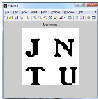
Figure 2: Logo image
