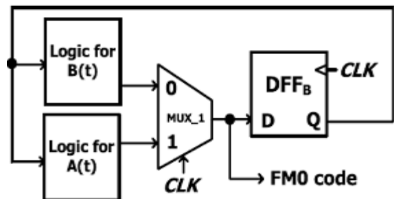
FM0 encoding without area compact retiming
