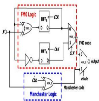
Hardware architecture
